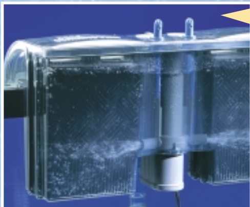
Venturi action across BioGrid™ as seen from the back of filter.
